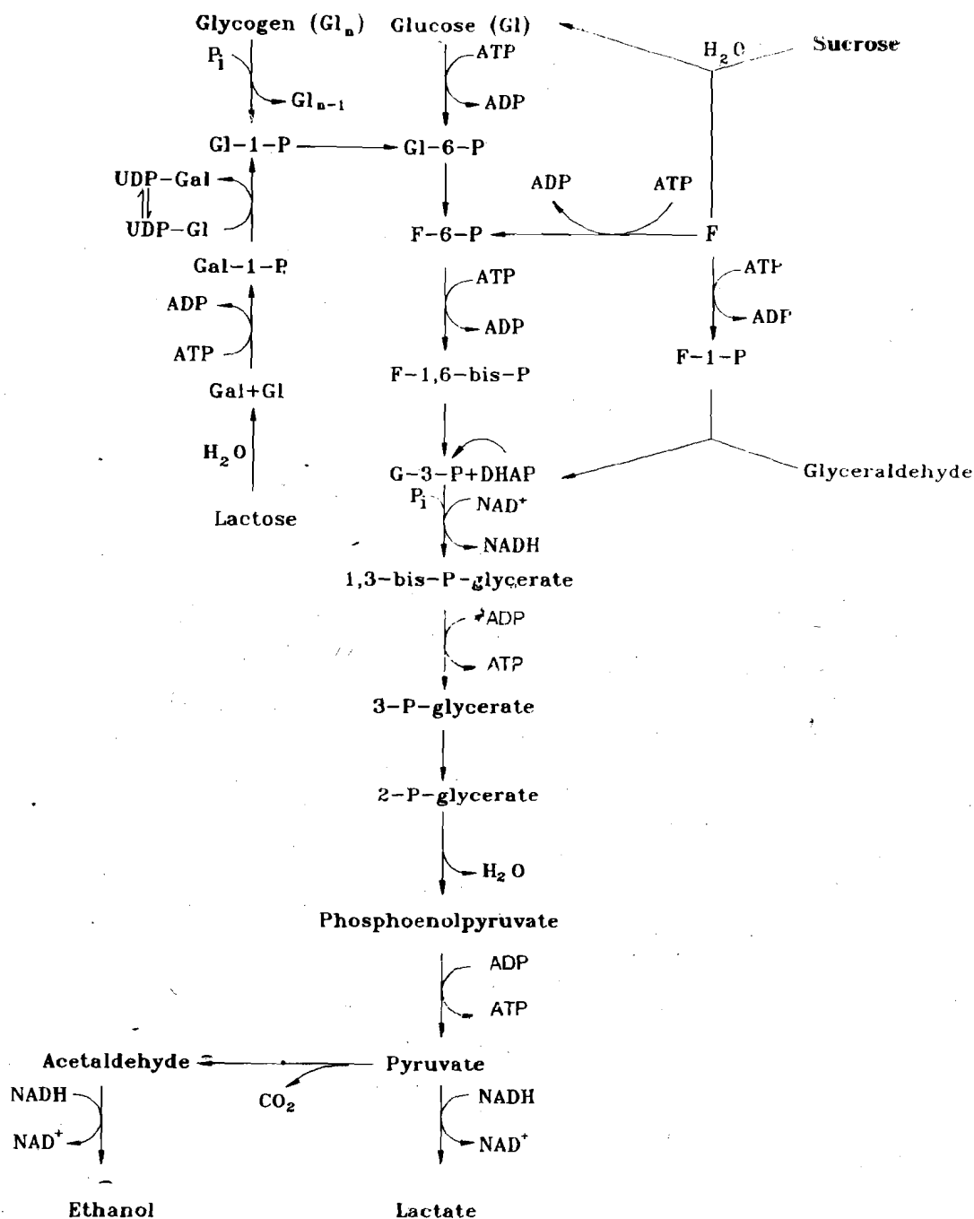
Fig. 9.2 : Scheme of glycolysis and alcoholic fermentation showing entry points for various sugars. The brown arrows are shown for the irreversible reactions. Abbreviations: Glucose, Gl; Fructose, F; Phosphate group, P; Phosphate ion, P i ; Glyceraldehyde-3-phosphate, G-3-P; Dihydroxyacetonephosphate, DHAP; Galactose Gal.
